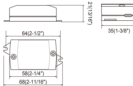
Dimensions: (mm/inches)
